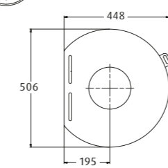
WESTFIRE.UNIQ.45 (FORMERLY UNIQ 18) WEIGHT: 90 KG
