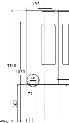
WESTFIRE.UNIQ.36 WESTFIRE.UNIQ.37 PEDESTAL 1 / WEIGHT: 95 KG
