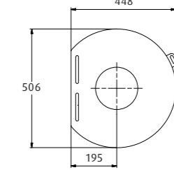
WESTFIRE.UNIQ.46 (FORMERLY UNIQ 18 WITH LOGDOOR) WEIGHT: 90 KG
