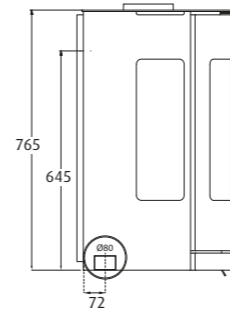
WESTFIRE.UNIQ.36 WESTFIRE.UNIQ.37 WALL-MOUNTED / WEIGHT: 85 KG
